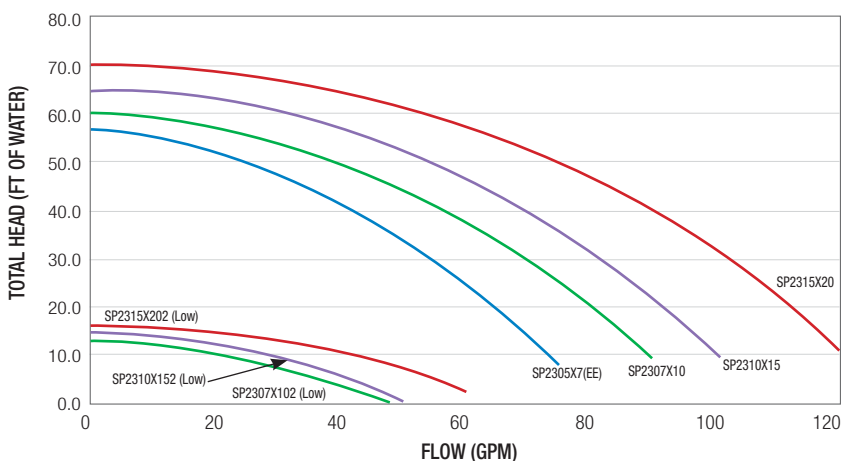
MAX-FLO XL FLOW VS TOTAL HEAD
