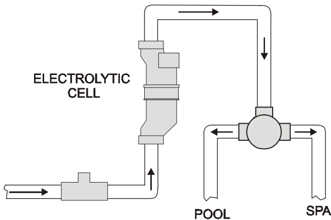
Vertical Installation
