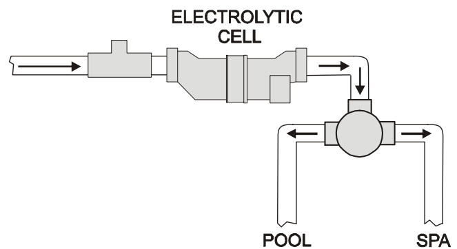
Inverted Installation
